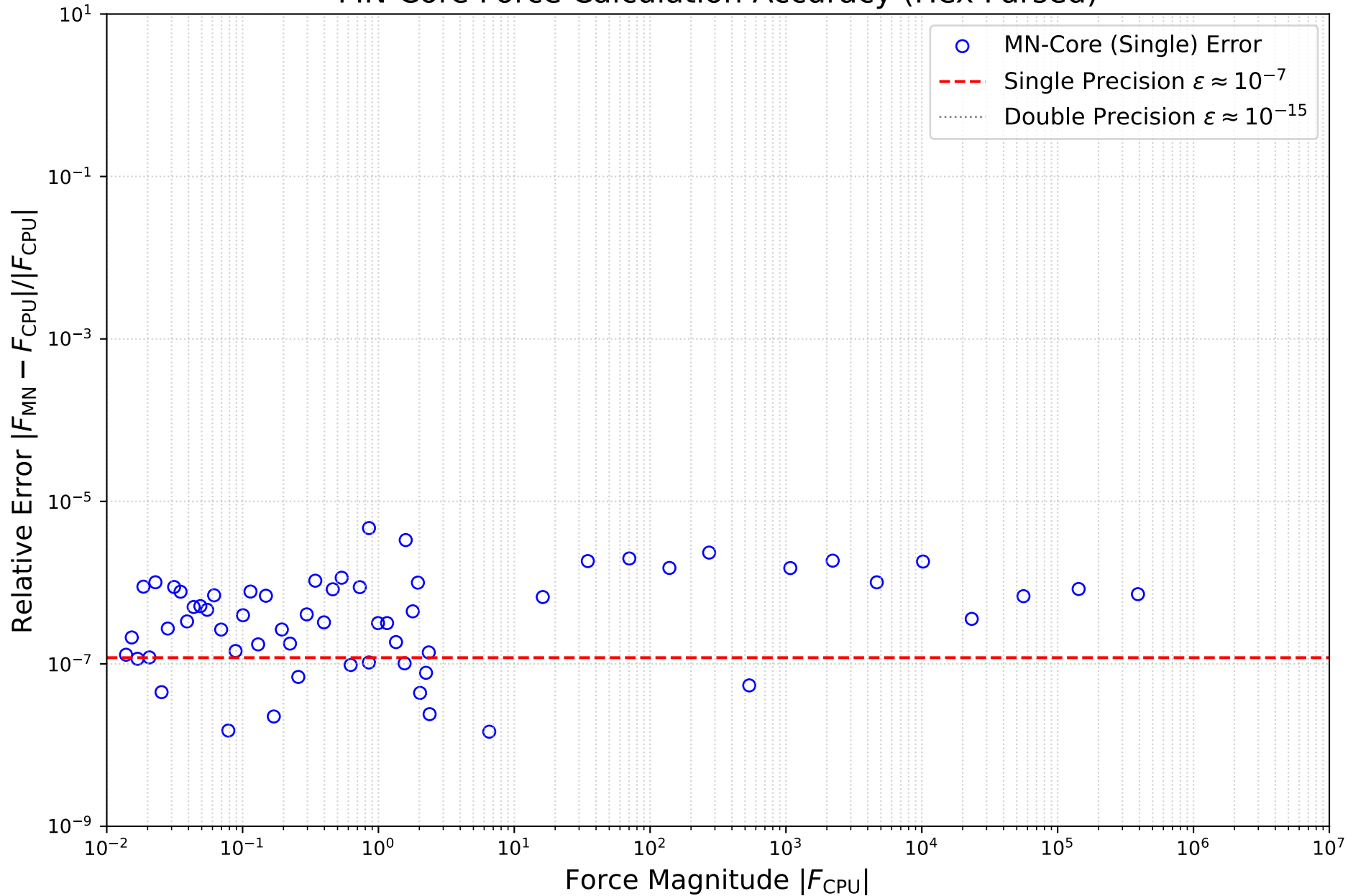
MN-Core Force Calculation Accuracy (Hex Parsed)
