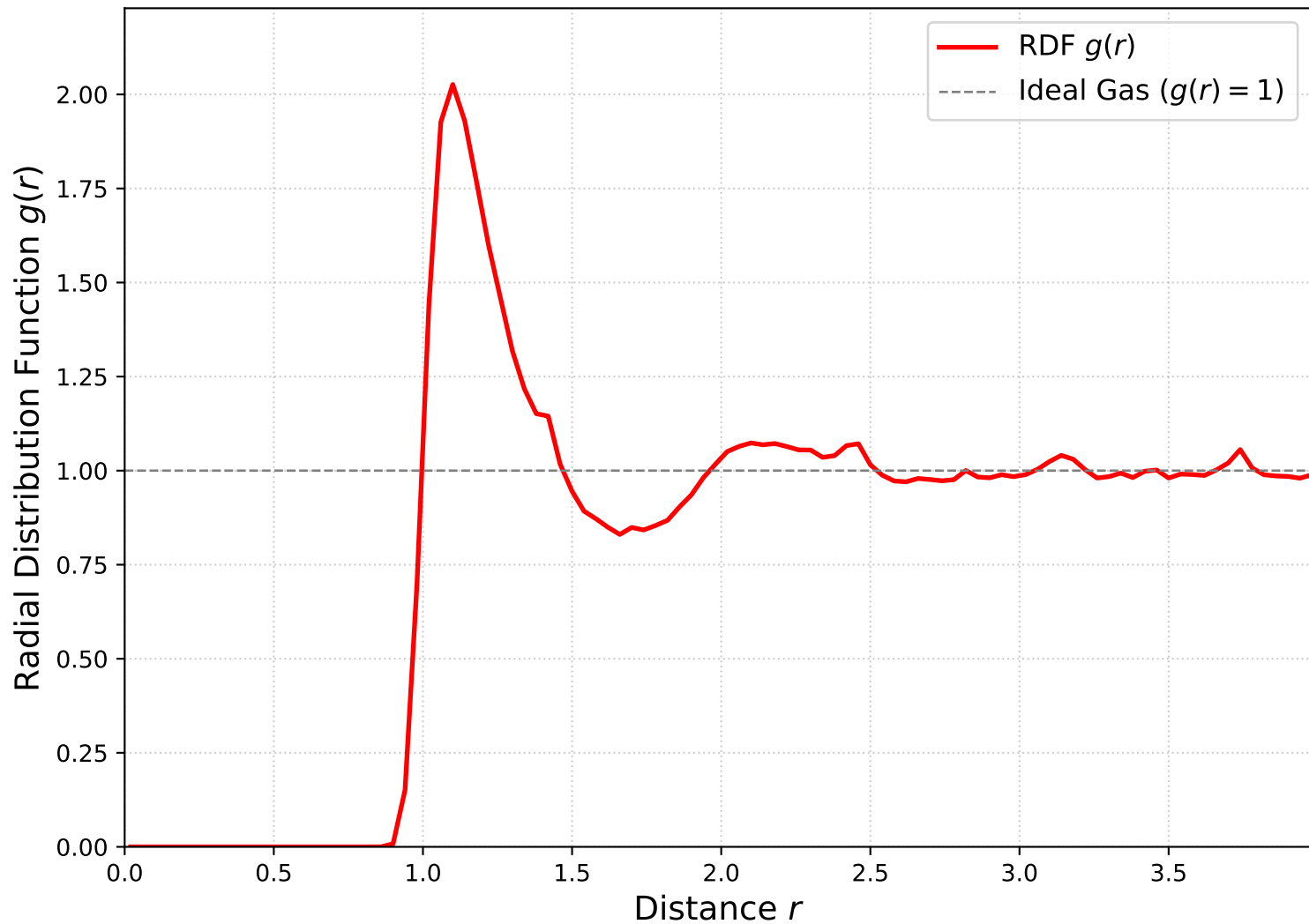
Radial Distribution Function (Liquid \rho \approx 0.5 )
