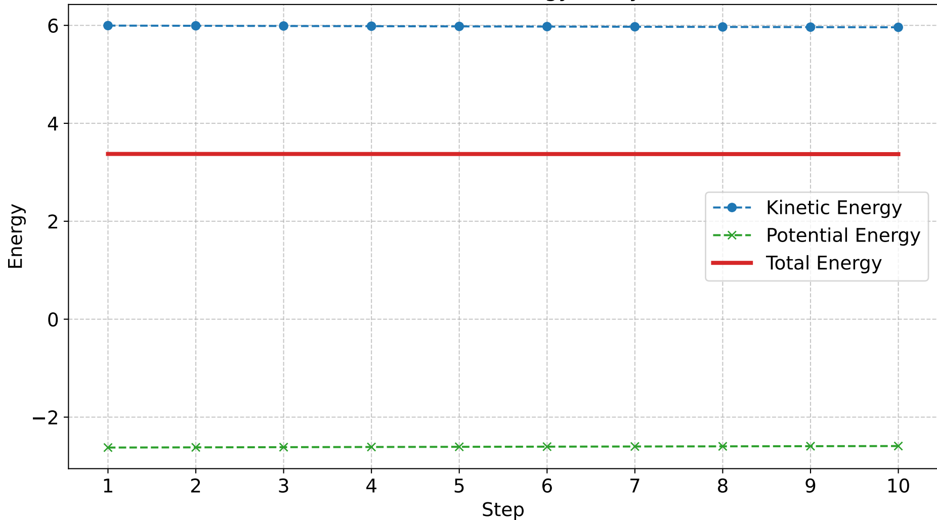
4-Particle MD Energy Analysis
