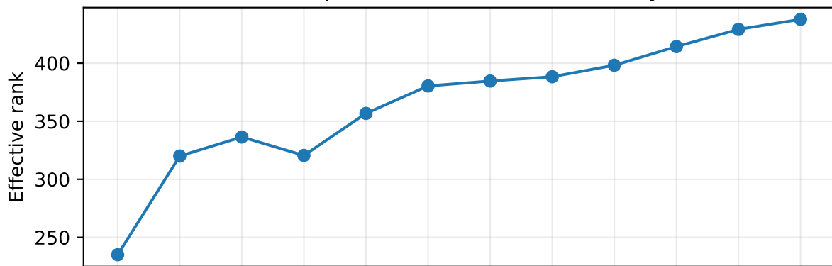
(b) Representational dimensionality
