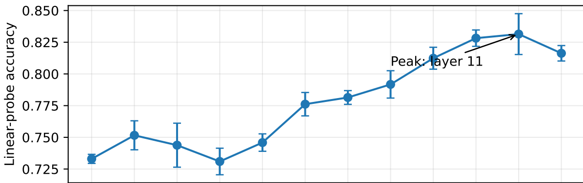
(a) Task-relevant information (mean \pm SD, 5 seeds)
