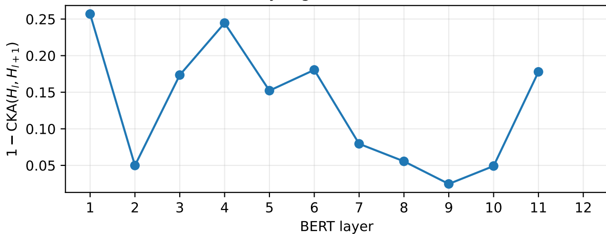
(c) Inter-layer geometric deformation
