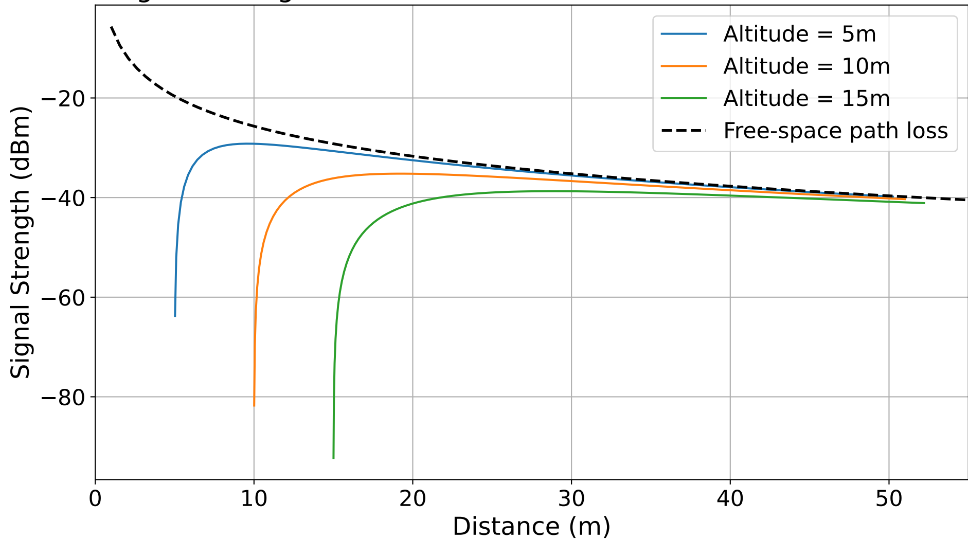
Signal Strength vs Distance at 915MHz for Different Altitudes
