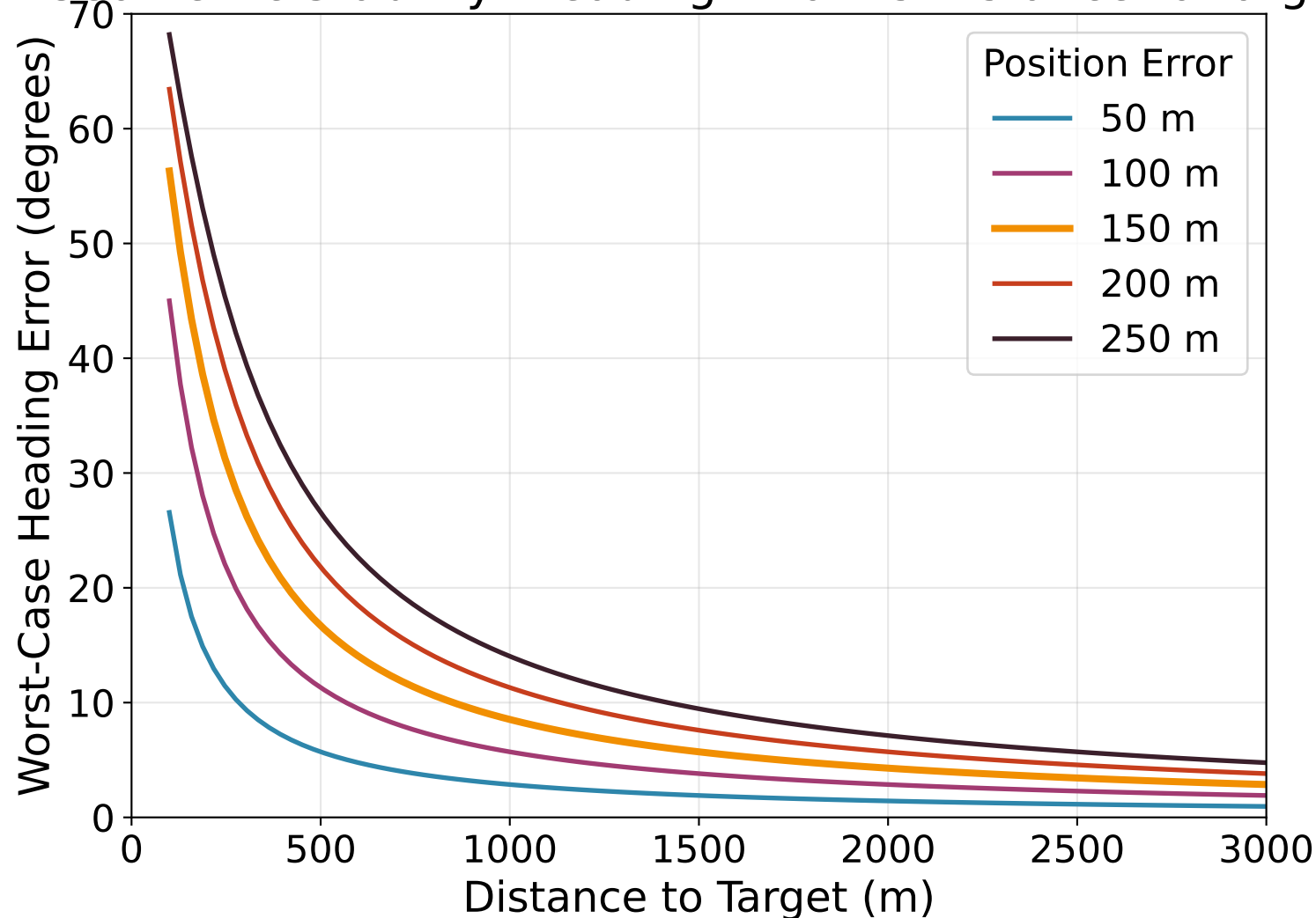
Geometric Stability: Heading Error vs Distance to Target
