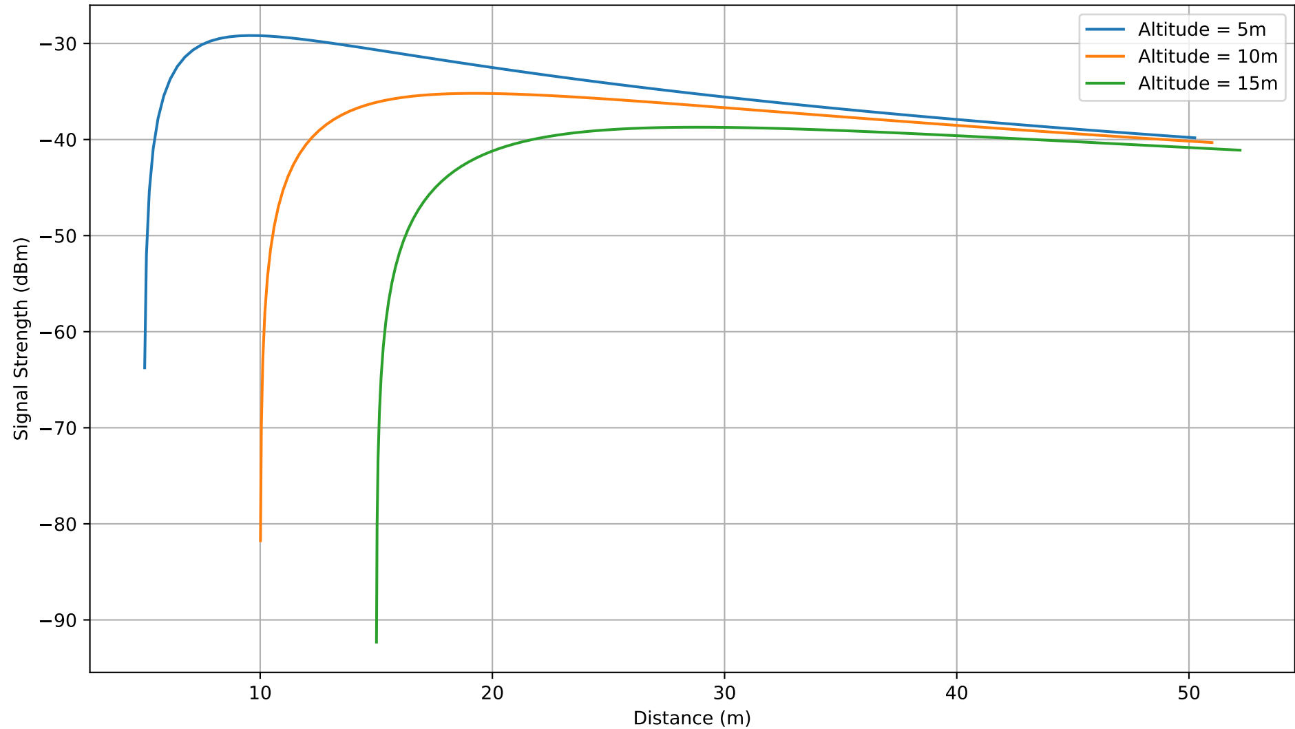
Signal Strength vs Distance at 915MHz for Different Altitudes
