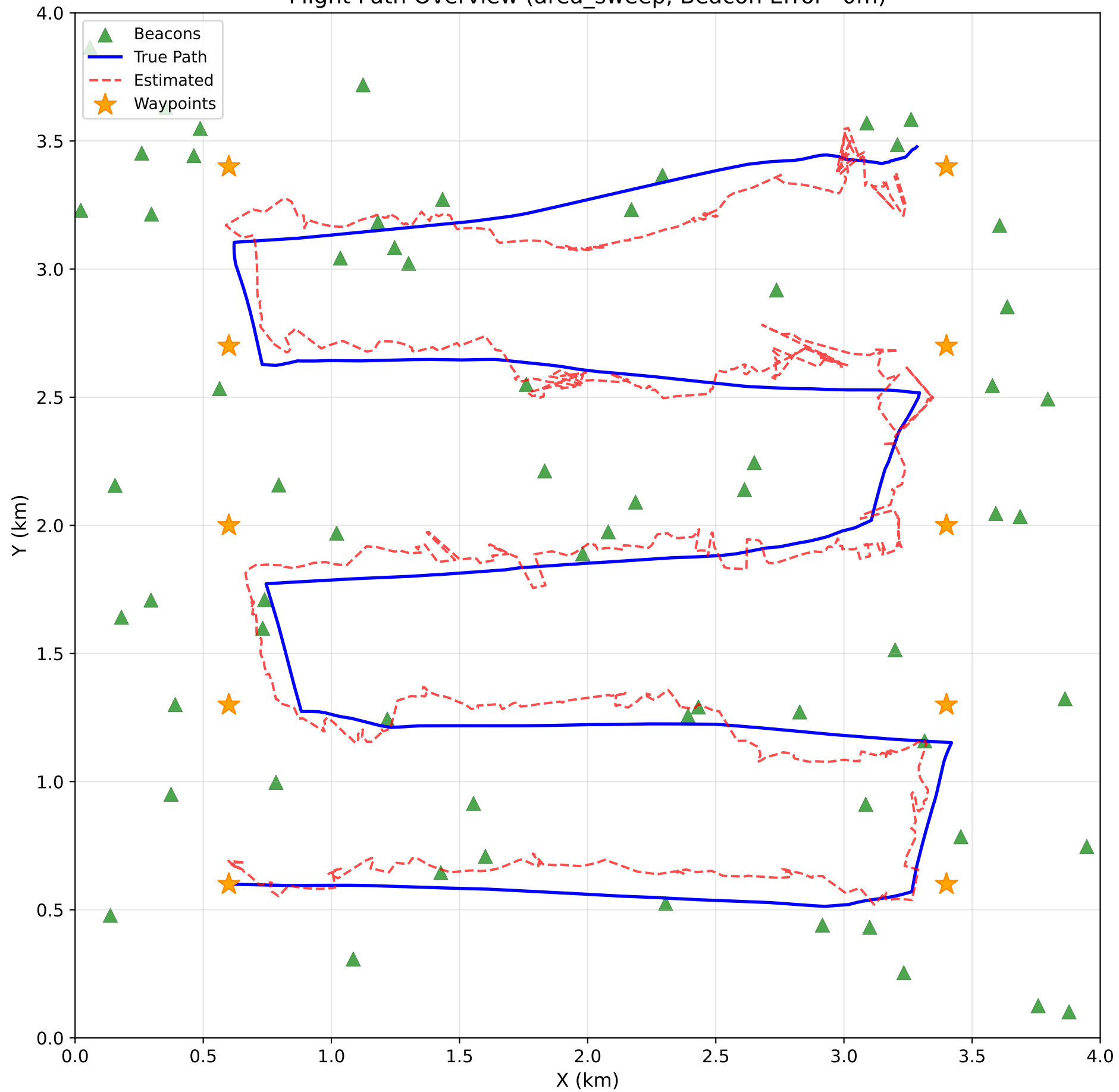
Flight Path Overview (area_sweep, Beacon Error=0m)
