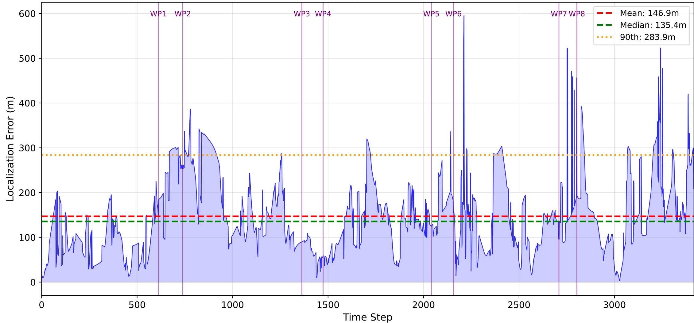
Error During Flight (area_sweep, Beacon Error=200m)
