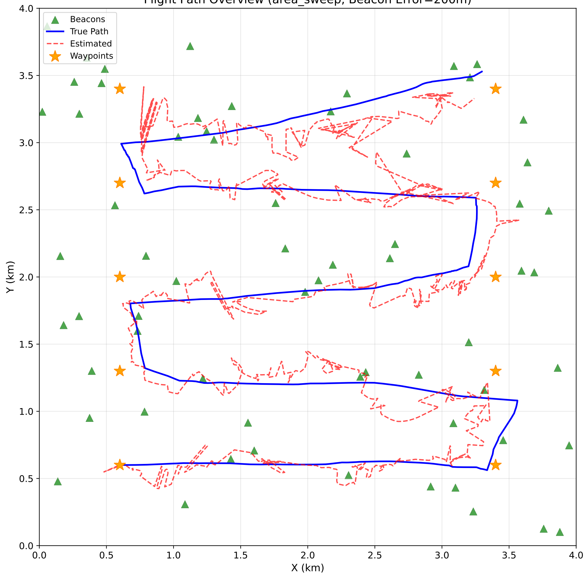
Flight Path Overview (area_sweep, Beacon Error=200m)
