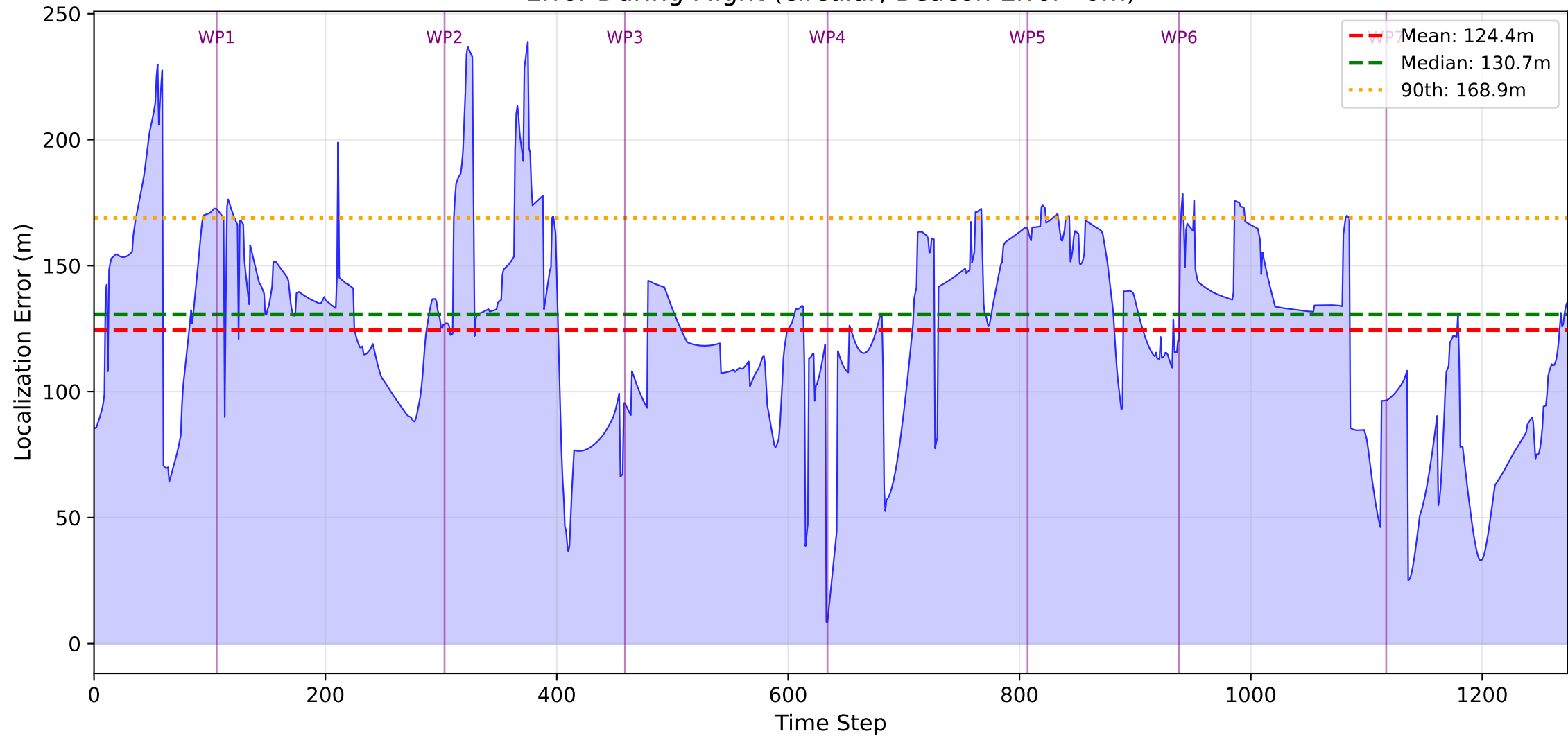
Error During Flight (circular, Beacon Error=0m)
