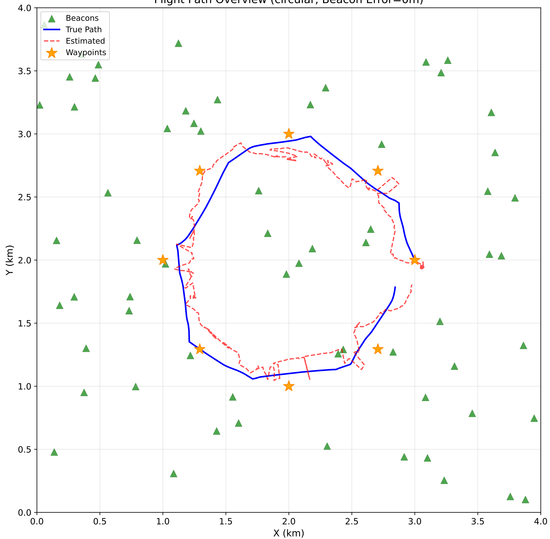
Flight Path Overview (circular, Beacon Error=0m)
