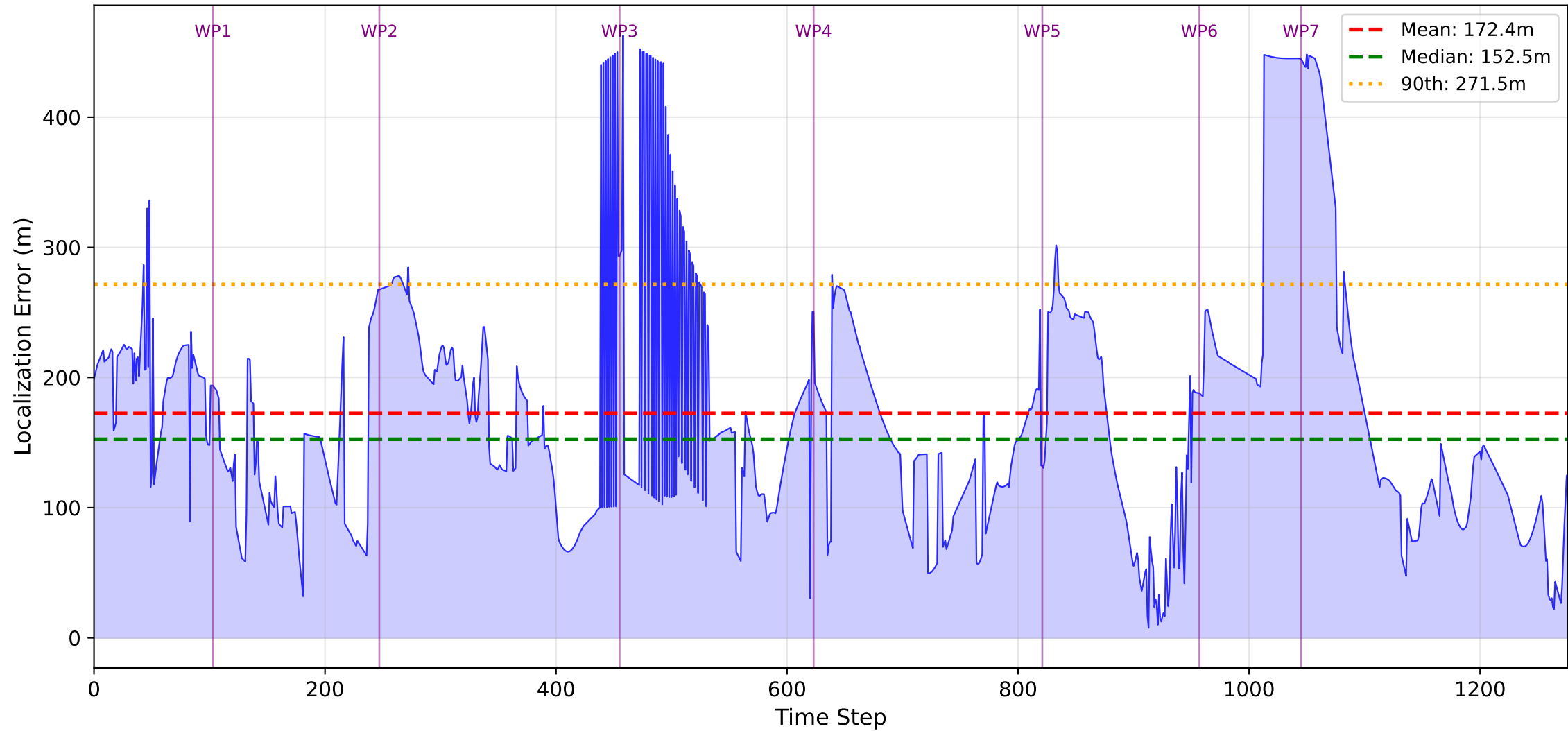
Error During Flight (circular, Beacon Error=200m)
