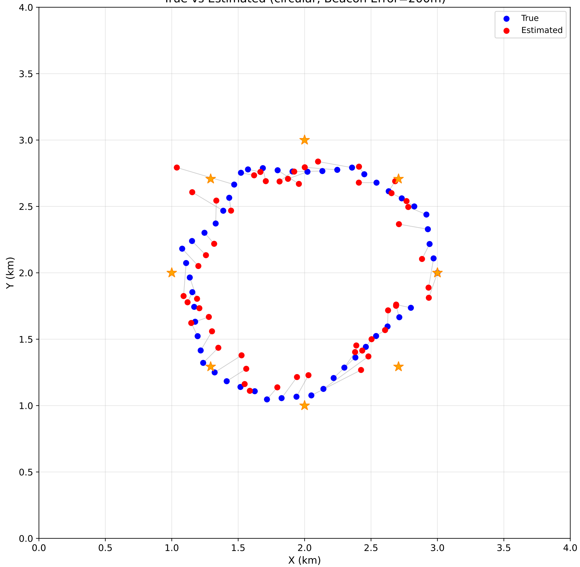
True vs Estimated (circular, Beacon Error=200m)
