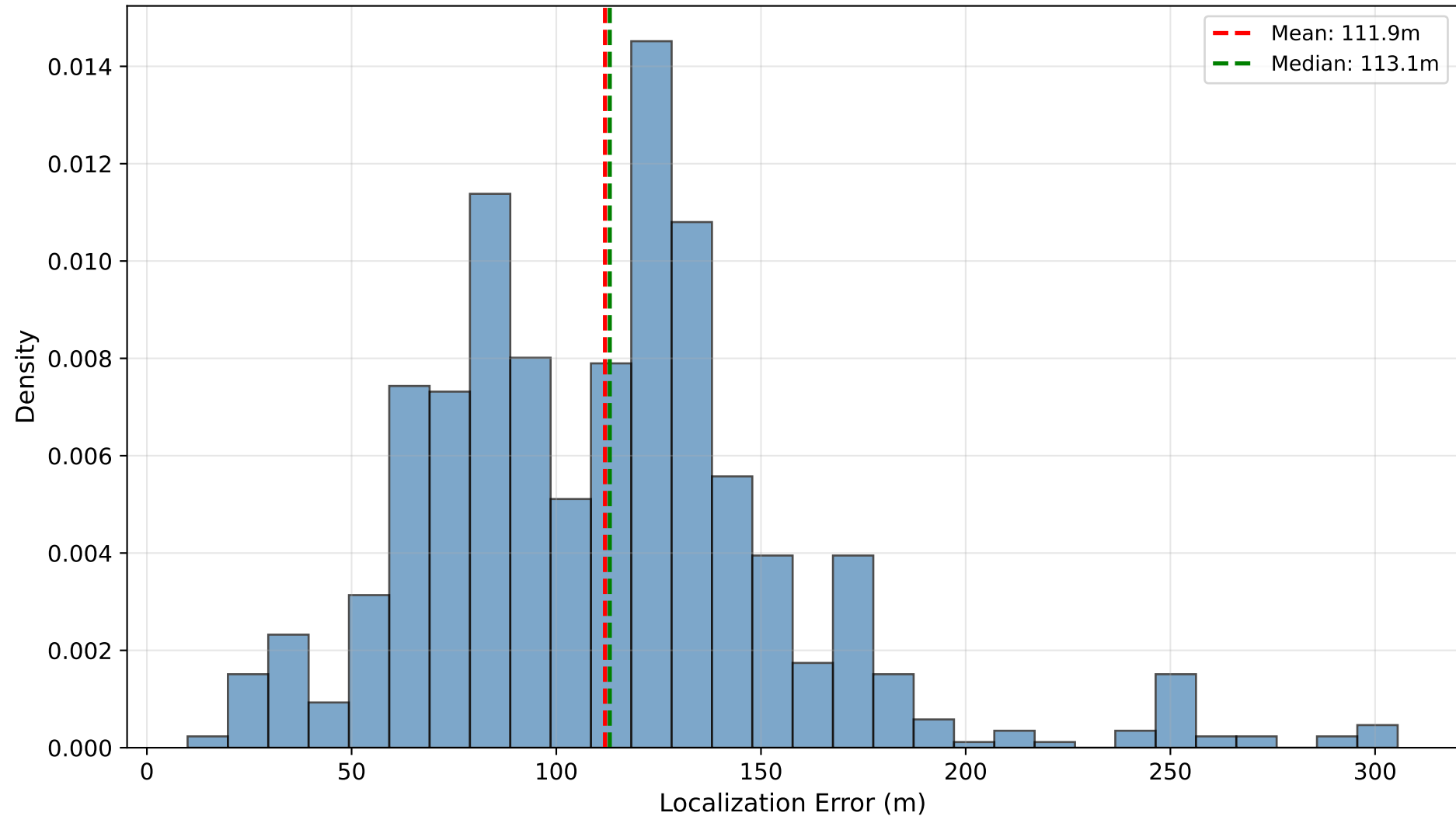
Error Distribution (diagonal, Beacon Error=0m)
