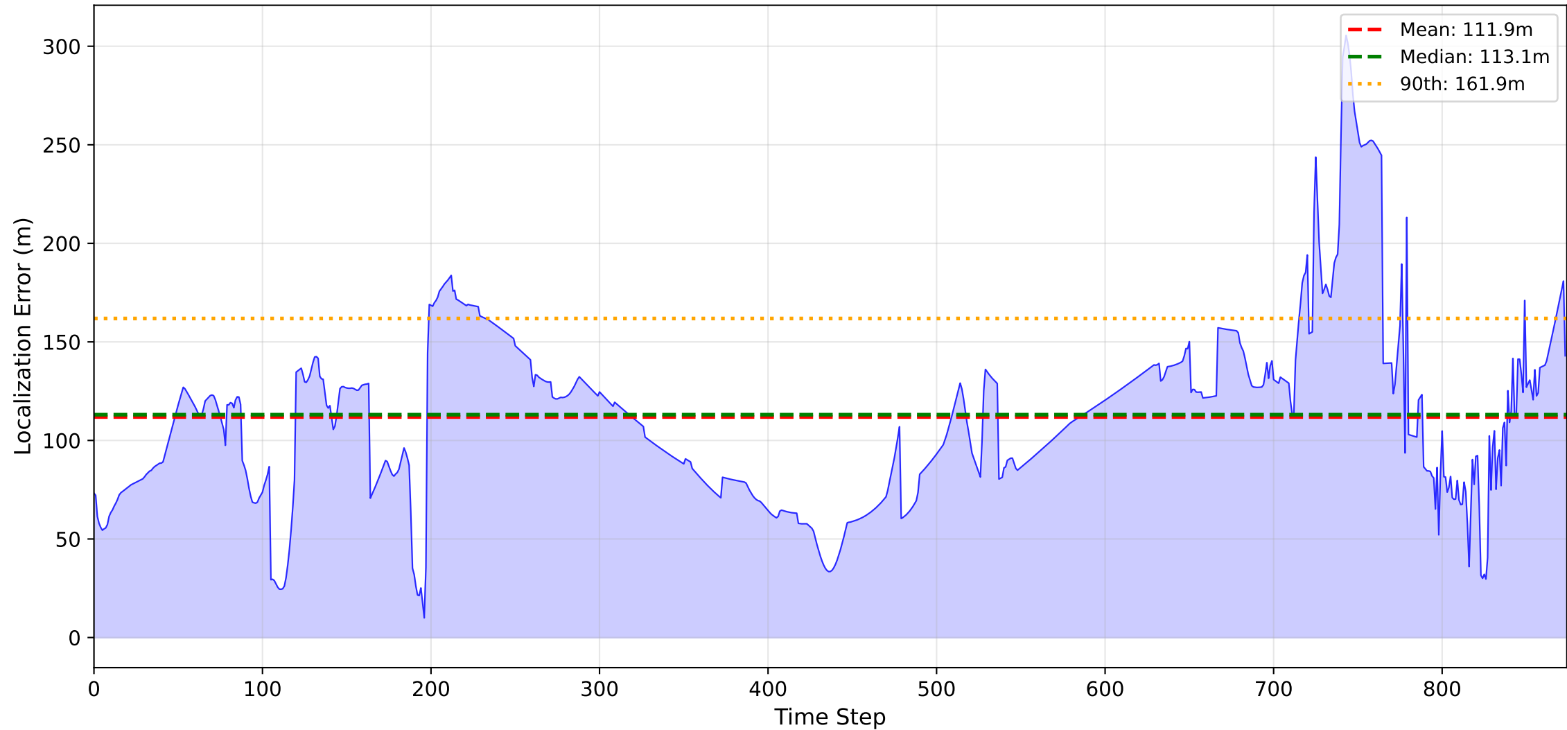
Error During Flight (diagonal, Beacon Error=0m)
