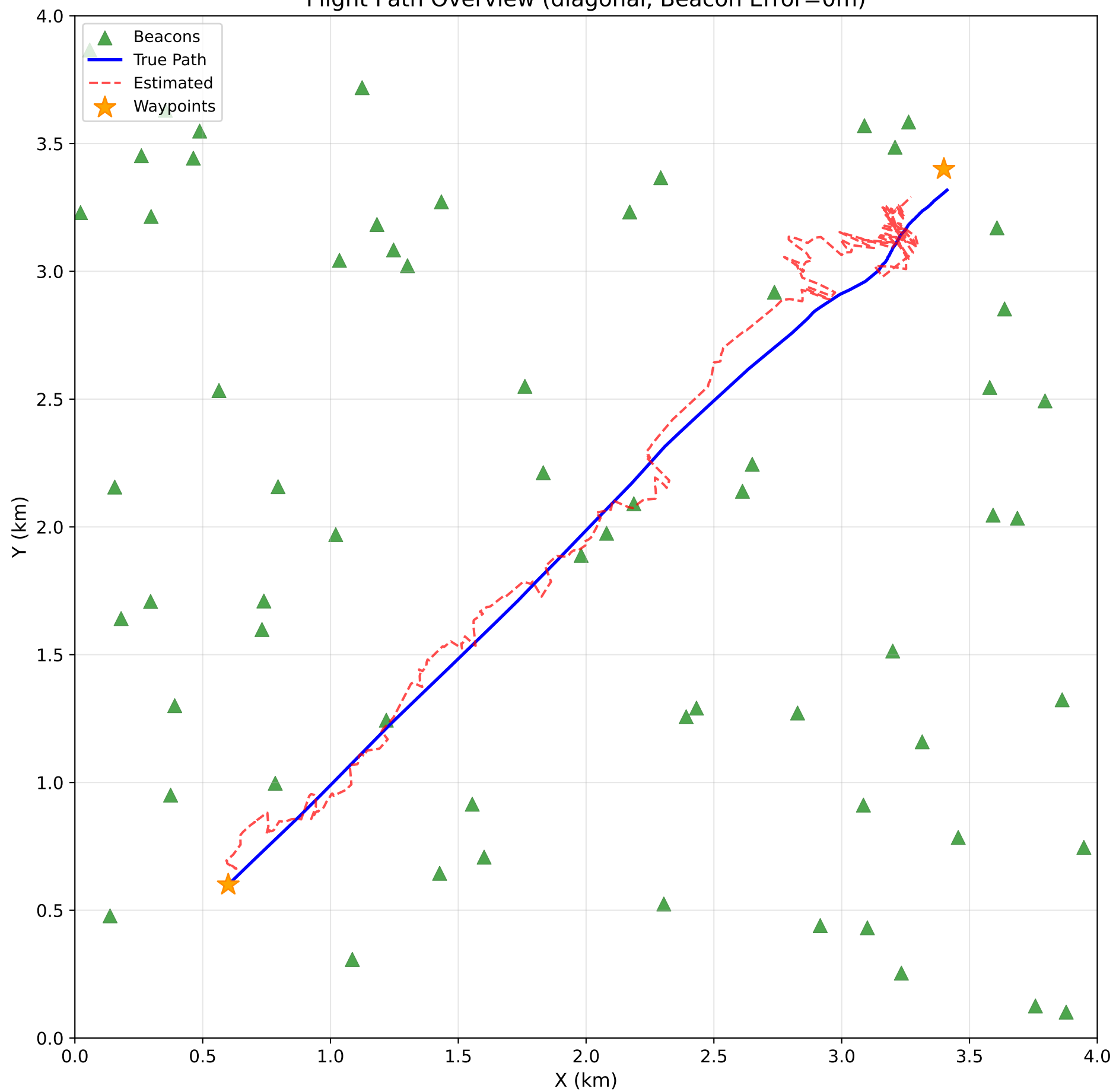
Flight Path Overview (diagonal, Beacon Error=0m)
