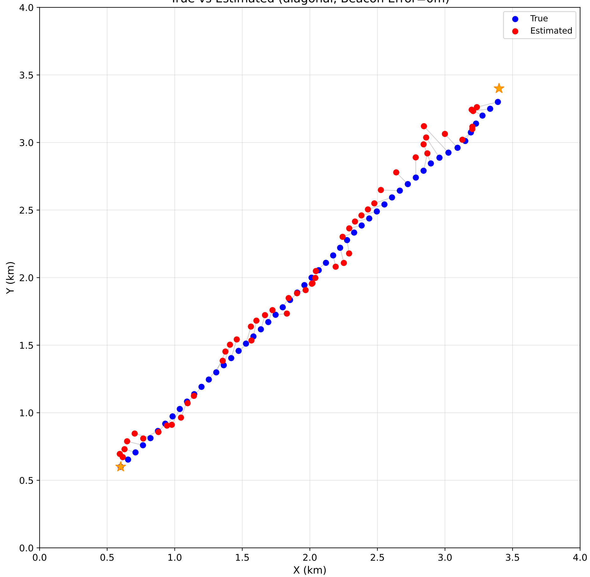
True vs Estimated (diagonal, Beacon Error=0m)
