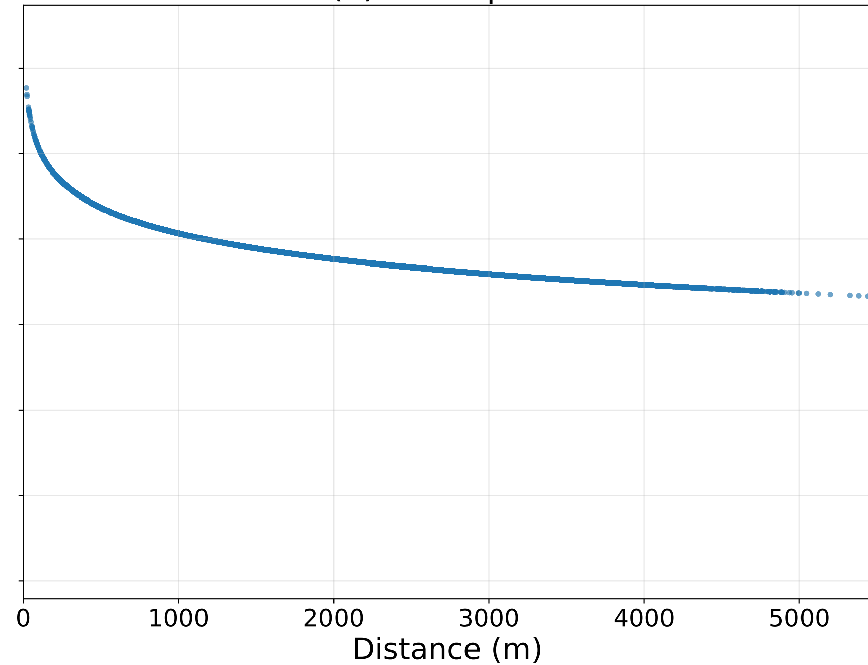
(b) Free-Space
