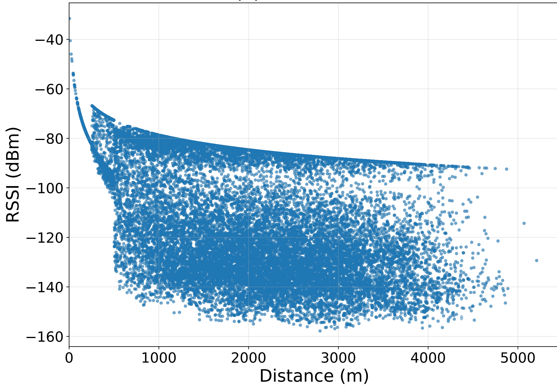
(a) Terrain-Aware
