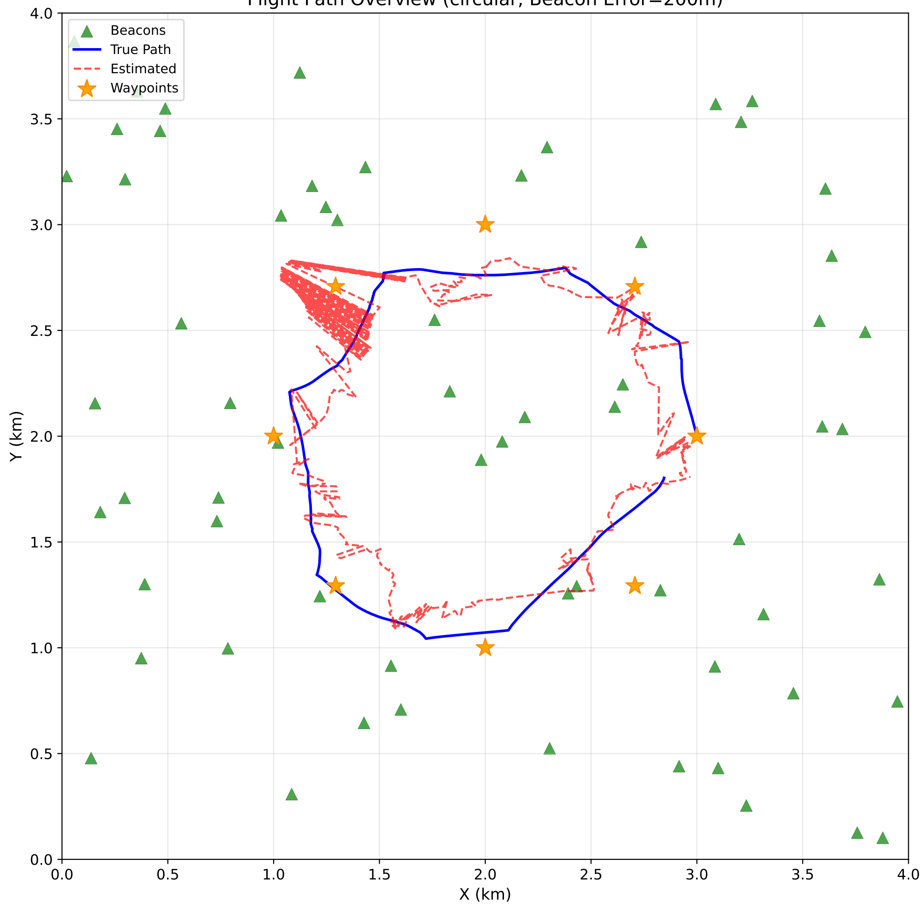
Flight Path Overview (circular, Beacon Error=200m)
