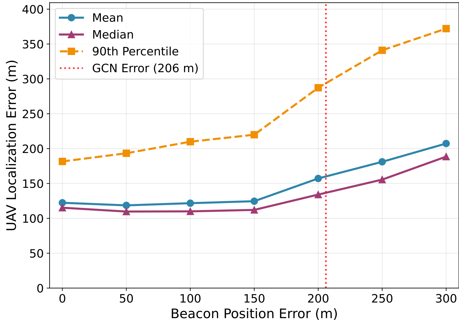
UAV Localization Error vs Beacon Position Error
