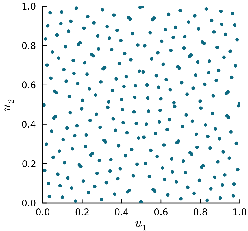
Sobol sequence
