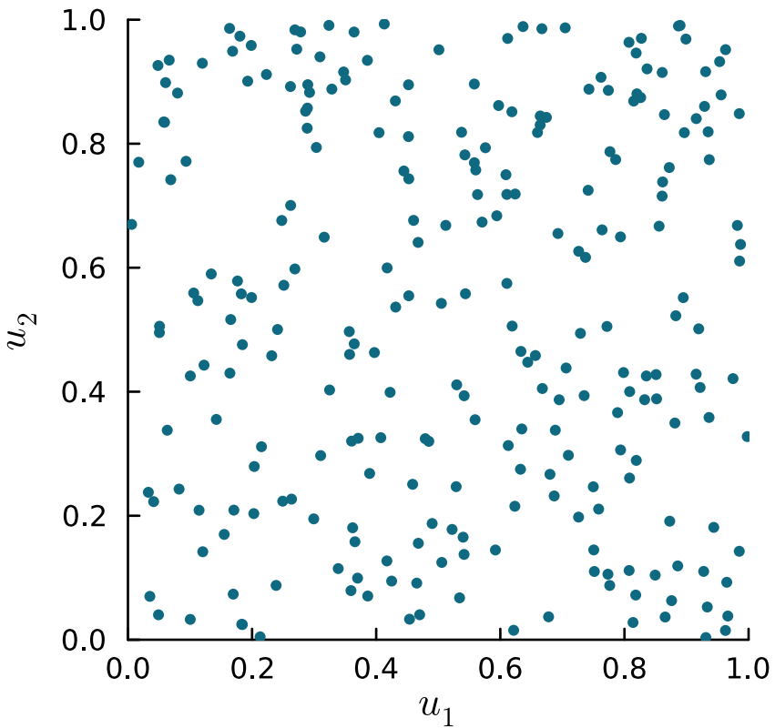
Pseudo-random
