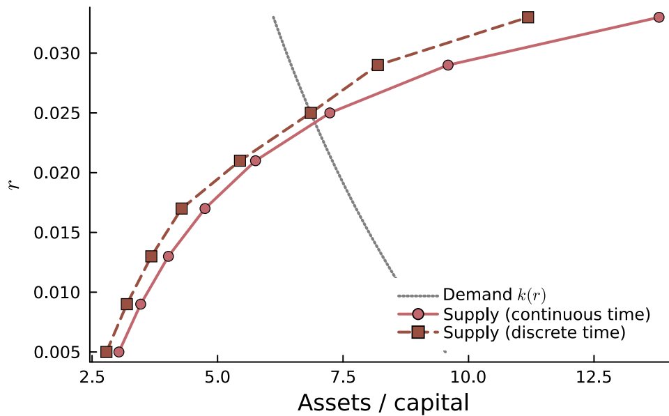
図 B.7: Capital demand and supply. Continuous vs. discrete time, same calibration.
