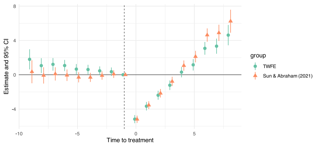
図 8.3: Event-study estimates on staggered data: naive TWFE versus Sun and Abraham (2021).
