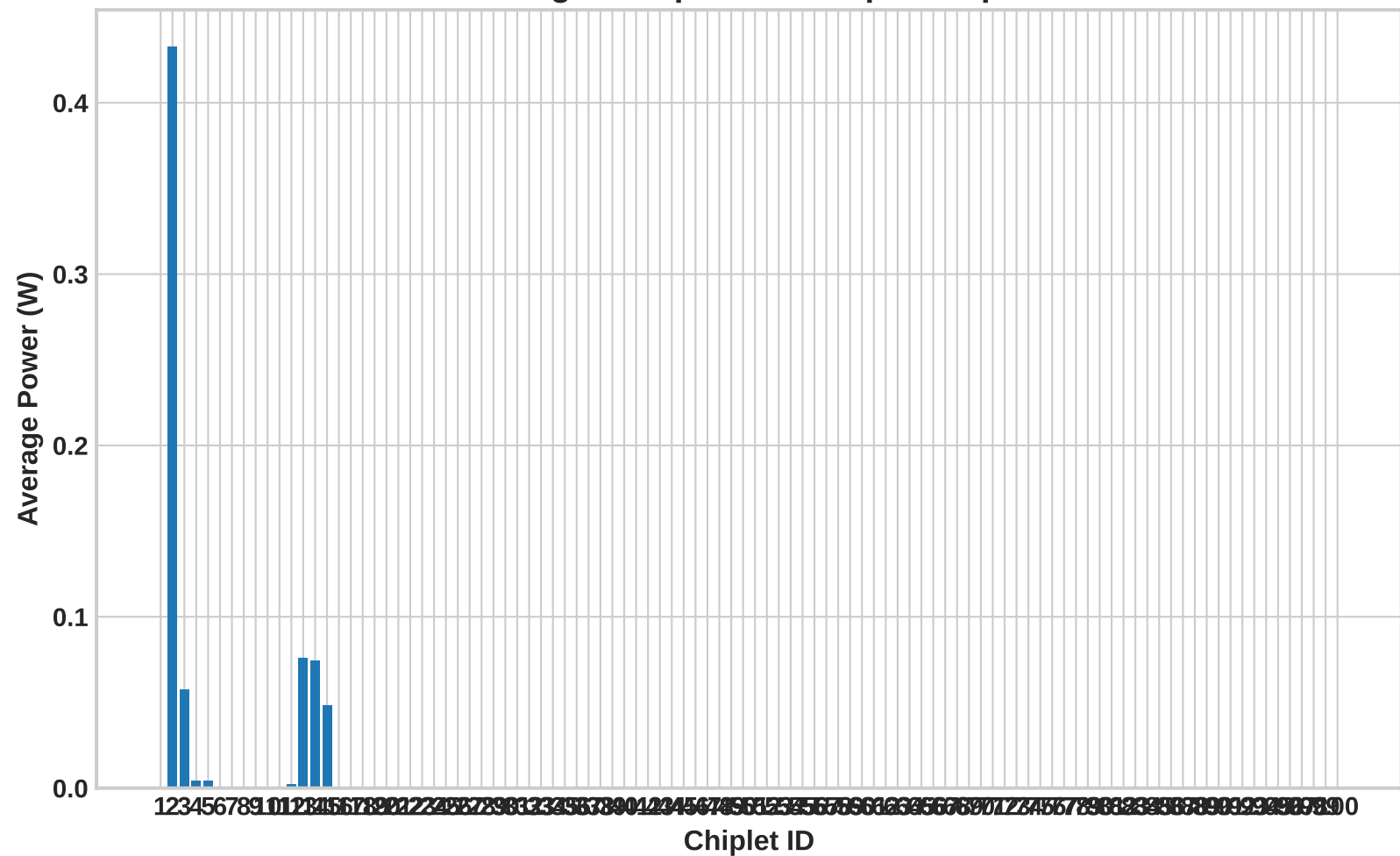
Average Compute Power per Chiplet
