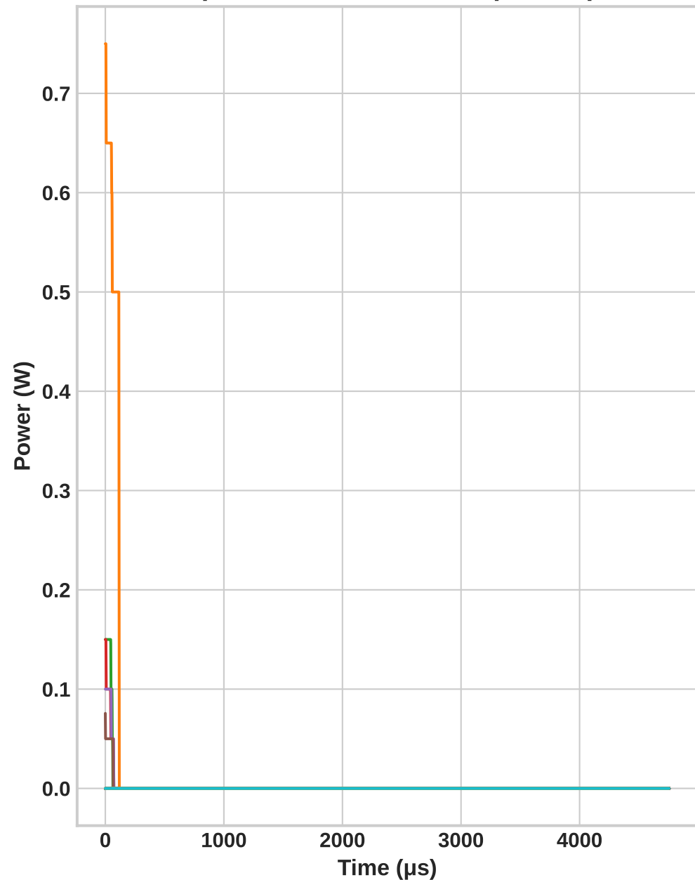
Chiplet 1 Chiplet 21 Chiplet 41 Chiplet 61 Chiplet 81 Chiplet 2 Chiplet 22 Chiplet 42 Chiplet 62 Chiplet 82 Chiplet 3 Chiplet 23 Chiplet 43 Chiplet 63 Chiplet 83 Chiplet 4 Chiplet 24 Chiplet 44 Chiplet 64 Chiplet 84 Chiplet 5 Chiplet 25 Chiplet 45 Chiplet 65 Chiplet 85 Chiplet 6 Chiplet 26 Chiplet 46 Chiplet 66 Chiplet 86 Chiplet 7 Chiplet 27 Chiplet 47 Chiplet 67 Chiplet 87 Chiplet 8 Chiplet 28 Chiplet 48 Chiplet 68 Chiplet 88 Chiplet 9 Chiplet 29 Chiplet 49 Chiplet 69 Chiplet 89 Chiplet 10 Chiplet 30 Chiplet 50 Chiplet 70 Chiplet 90 Chiplet 11 Chiplet 31 Chiplet 51 Chiplet 71 Chiplet 91 Chiplet 12 Chiplet 32 Chiplet 52 Chiplet 72 Chiplet 92 Chiplet 13 Chiplet 33 Chiplet 53 Chiplet 73 Chiplet 93 Chiplet 14 Chiplet 34 Chiplet 54 Chiplet 74 Chiplet 94 Chiplet 15 Chiplet 35 Chiplet 55 Chiplet 75 Chiplet 95 Chiplet 16 Chiplet 36 Chiplet 56 Chiplet 76 Chiplet 96 Chiplet 17 Chiplet 37 Chiplet 57 Chiplet 77 Chiplet 97 Chiplet 18 Chiplet 38 Chiplet 58 Chiplet 78 Chiplet 98 Chiplet 19 Chiplet 39 Chiplet 59 Chiplet 79 Chiplet 99 Chiplet 20 Chiplet 40 Chiplet 60 Chiplet 80 Chiplet 100
