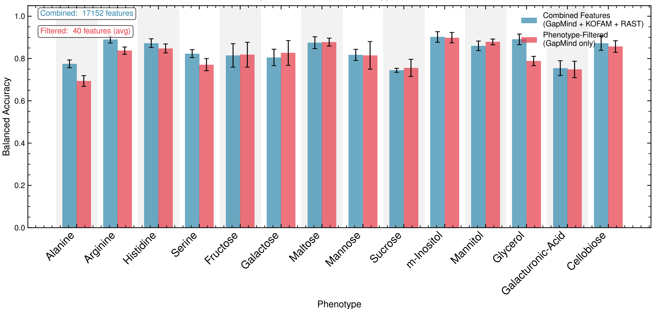
B. Dataset Split: Combined vs Phenotype-Filtered Features
