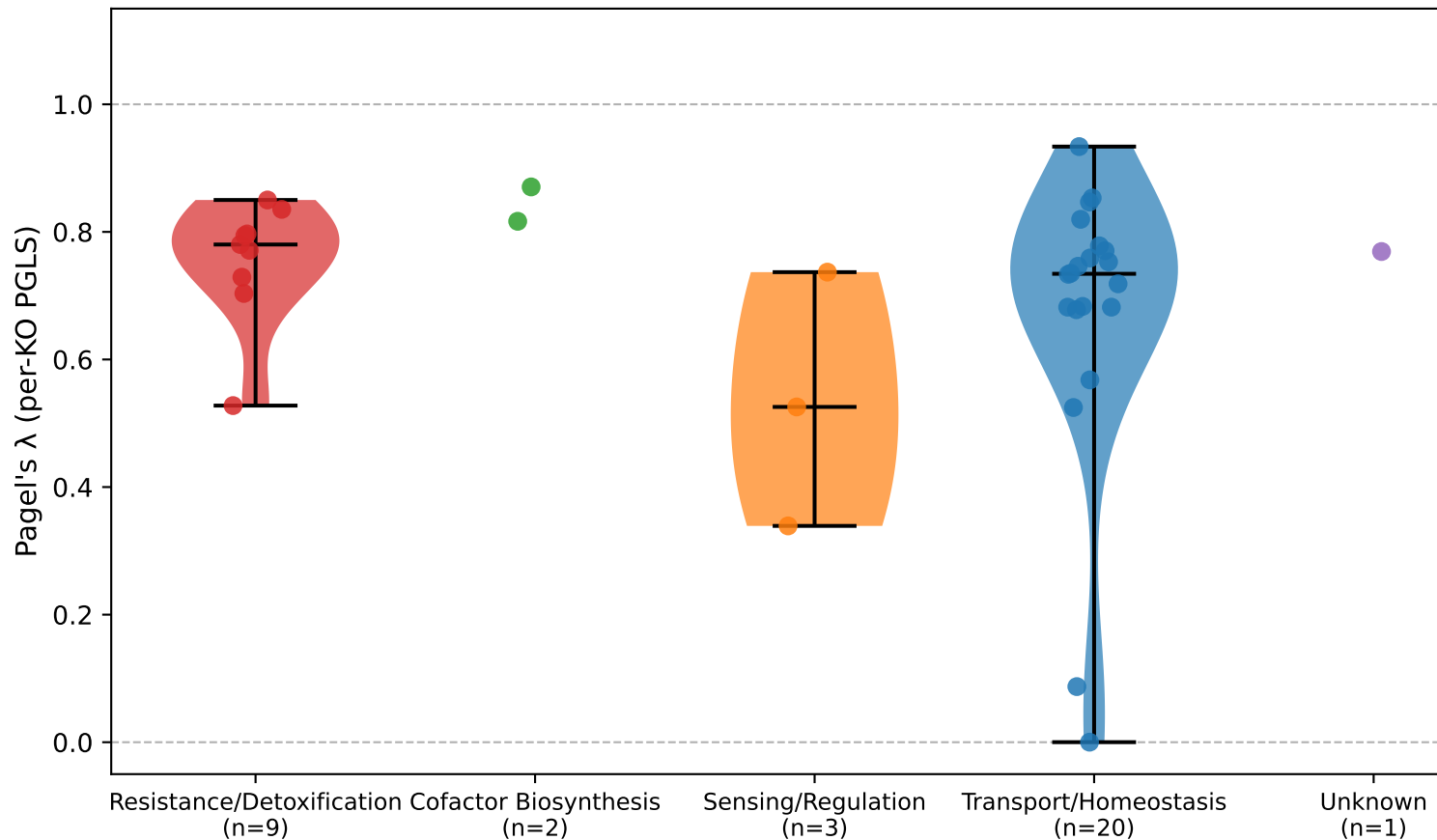
Phylogenetic signal ( \lambda ) per Tier 1+2 KO by functional subcategory
