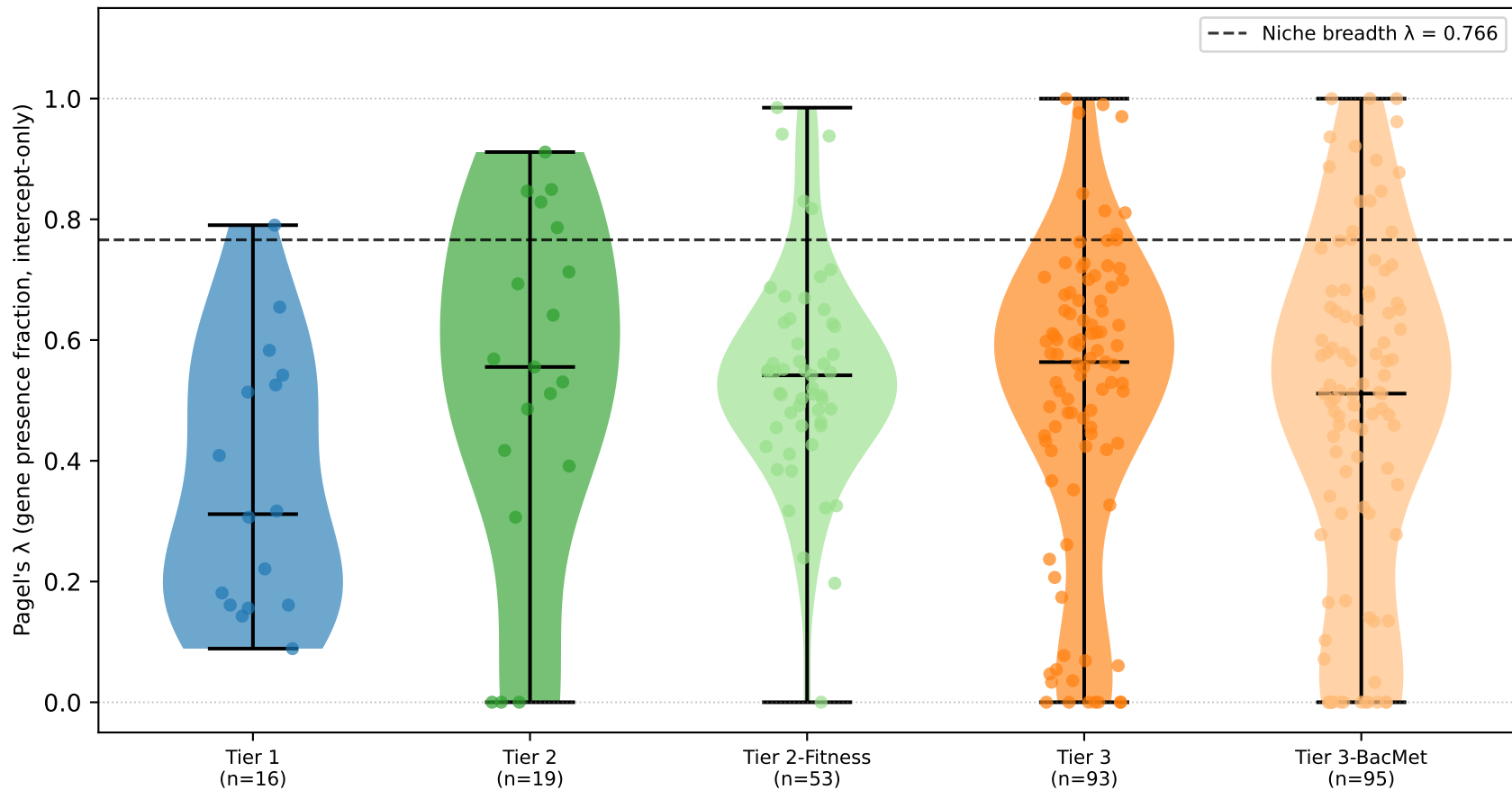
Phylogenetic signal by evidence tier — all curated metal KOs (n=276)
