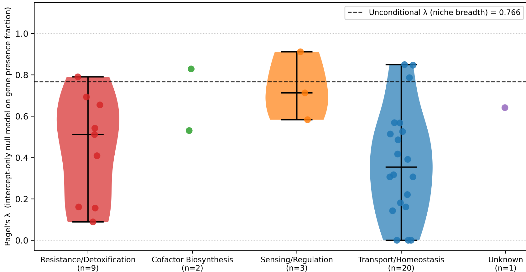
Phylogenetic signal of KO presence across genera — direct \lambda estimate
