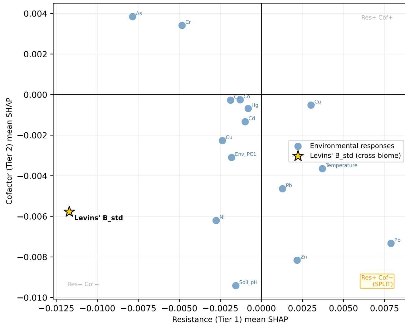
Resistance vs Cofactor SHAP direction across 16 response variables z-test p = 1.000
