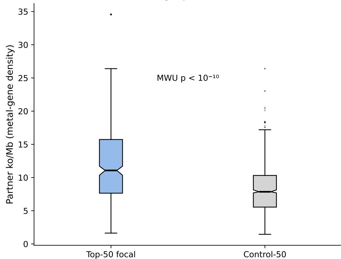
Fig C — Partner metal-gene density vs focal group (soil stratum)
