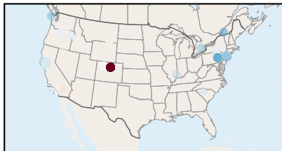
PC1 — lithogenic crustal (58% var.)
