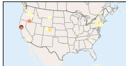
log(USGS Hg+1) — raw Hg (ppm)
