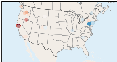
PC2 — Hg/hydrothermal (20% var.)
