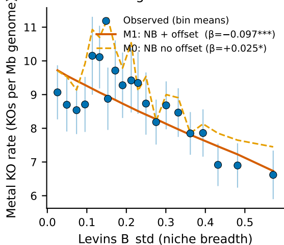
Absolute KO count \div genome size vs niche breadth
