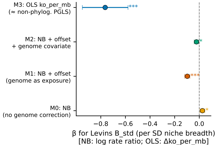
\beta across model specifications
