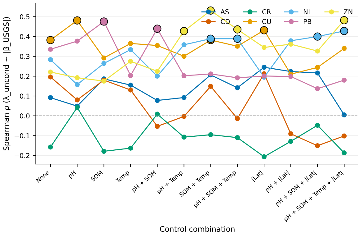
NB30 Fig 2: \lambda - \beta \rho trajectory per metal as controls added
