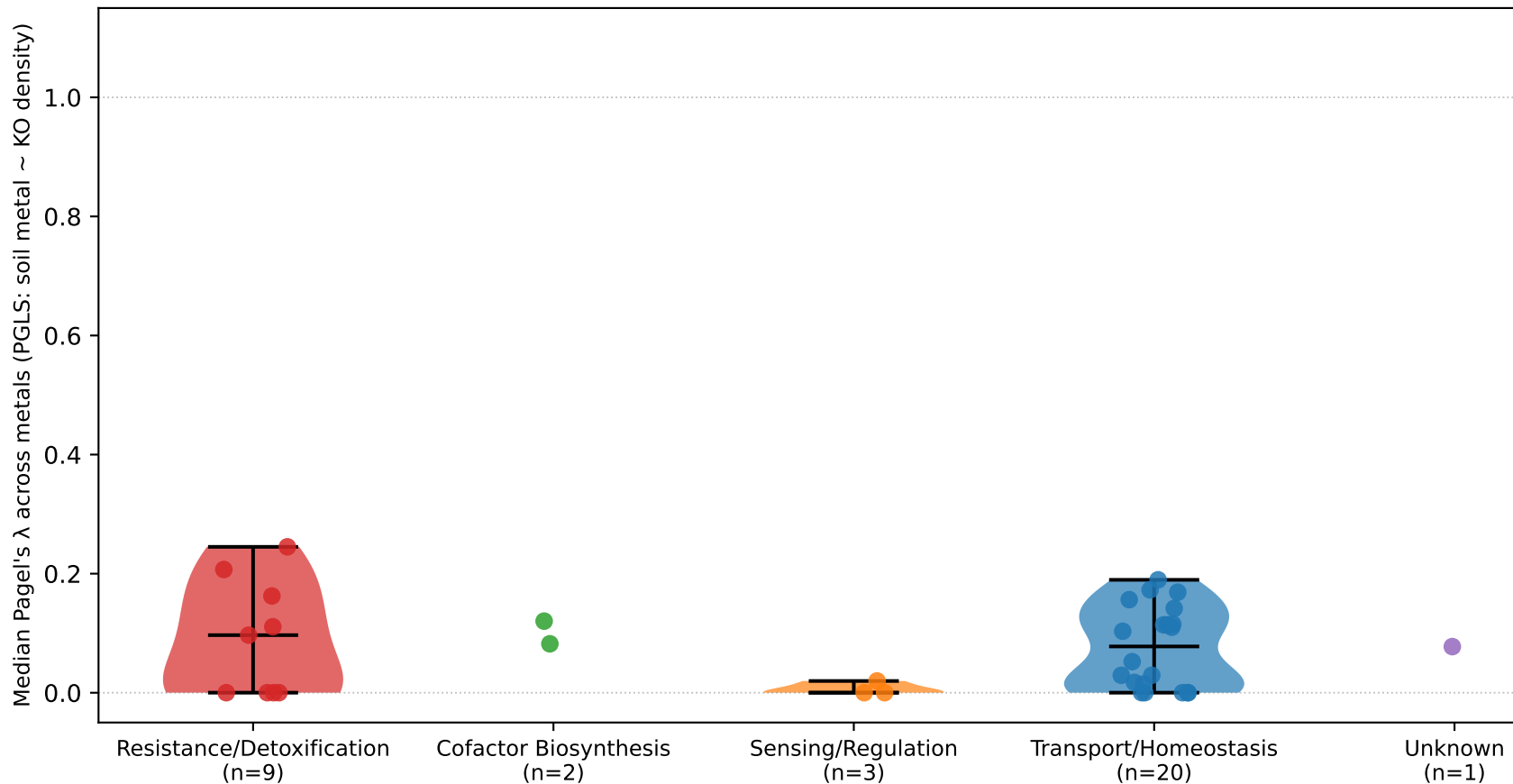
Per-KO \lambda by subcategory — GeoROC (bedrock)
