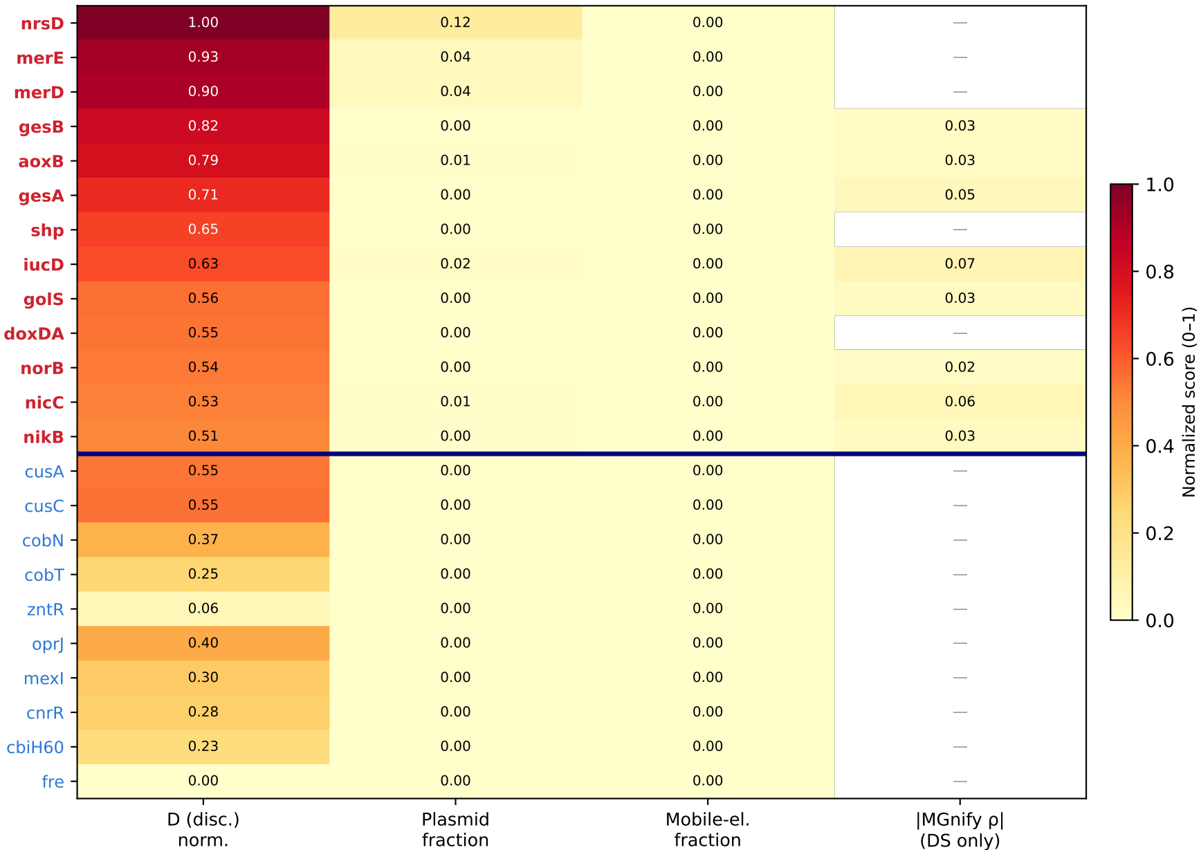
Fig C — HGT evidence heatmap per KO (red = high; — = not available)
