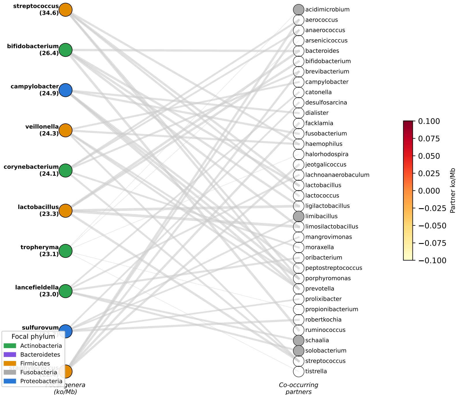
Fig A — Bipartite co-occurrence network (top-10 metal-gene-rich focal genera, top-5 partners by \phi , soil stratum)
