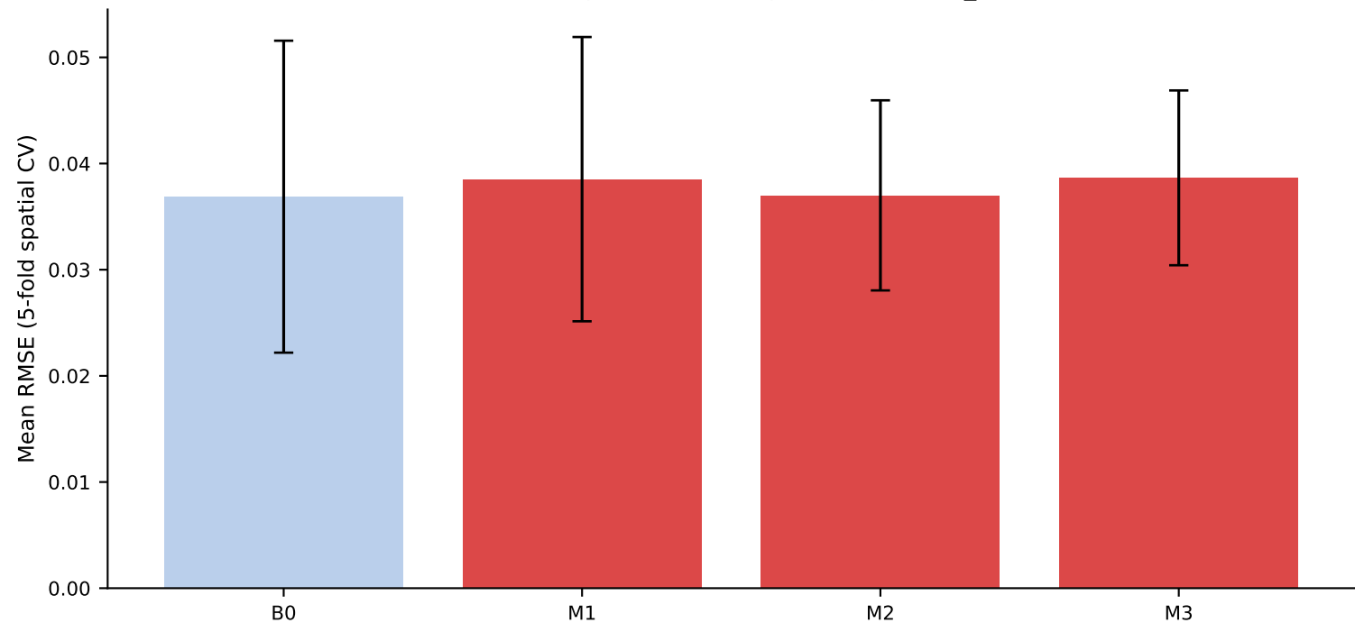
CV RMSE by model (MGnify) — target: PF1_Cu
