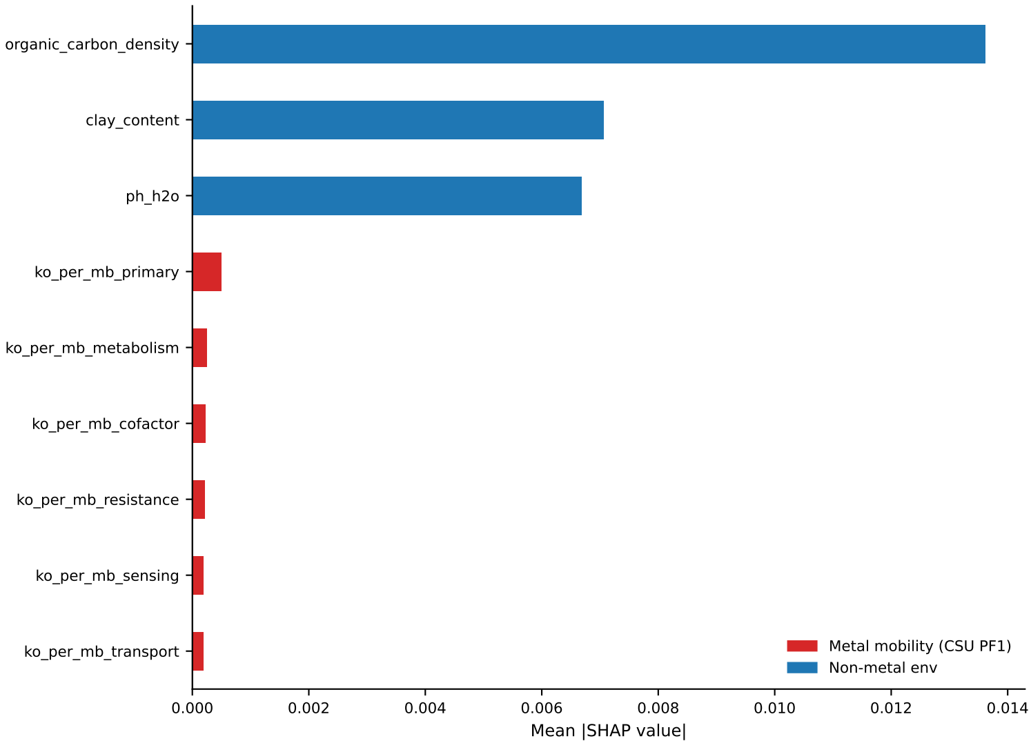
M3 SHAP importance (MGnify) — target: PF1_Cu
