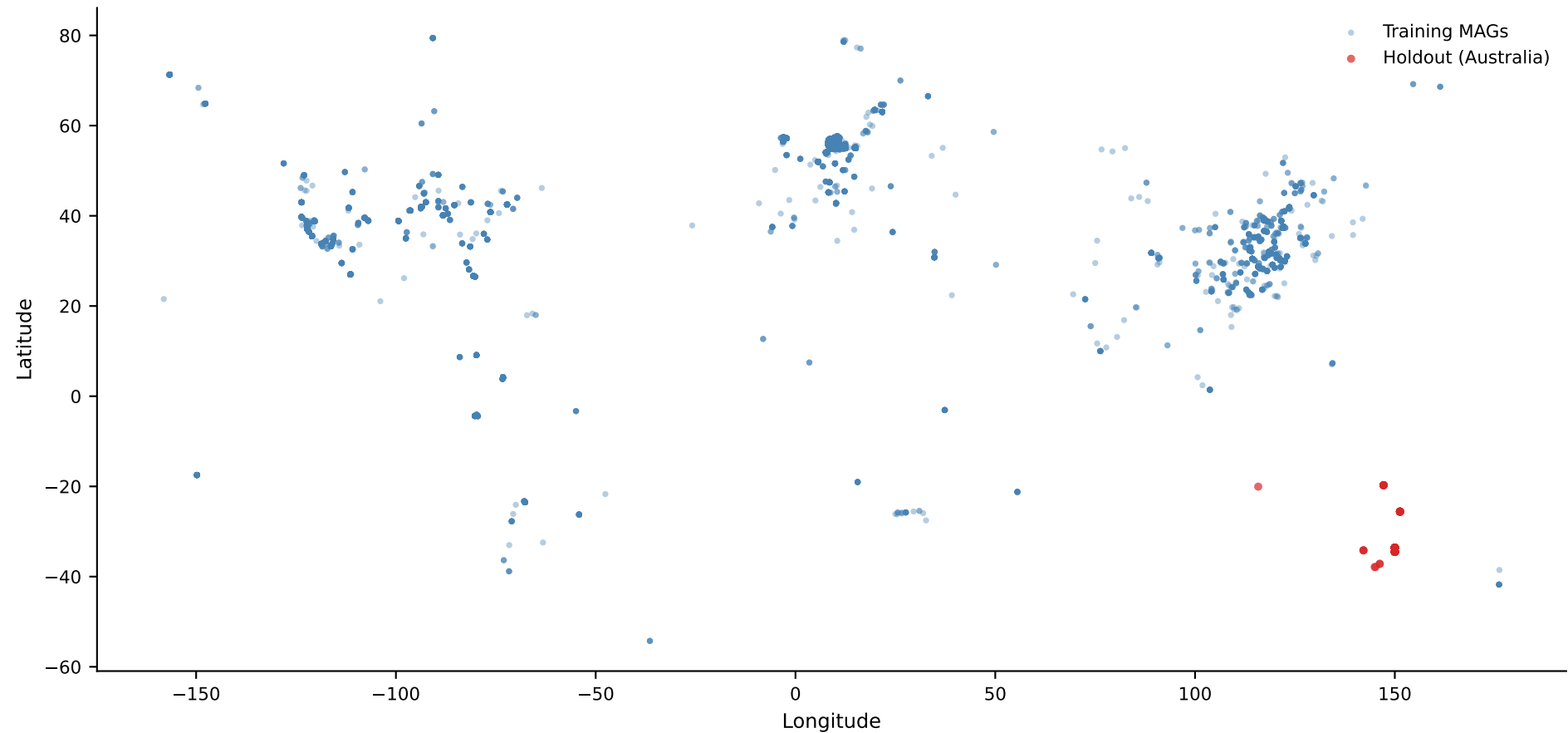
Geographic holdout — Australia (MGnify)
