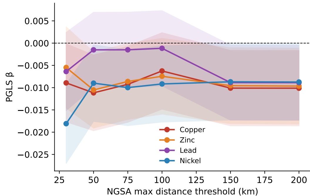
\beta coefficient stability across distance thresholds
