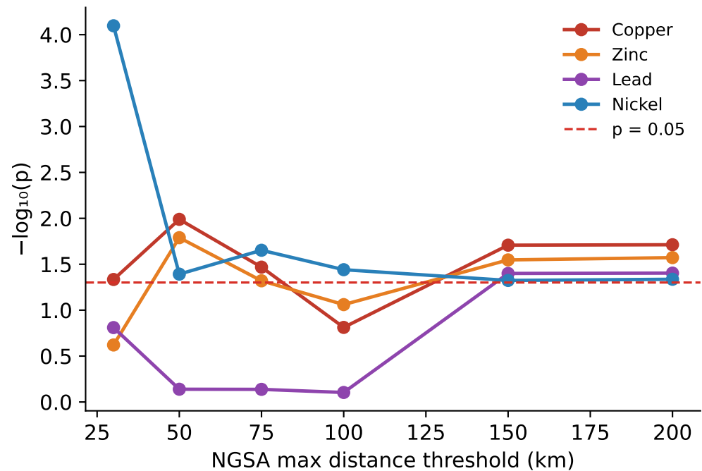
Significance stability across distance thresholds
