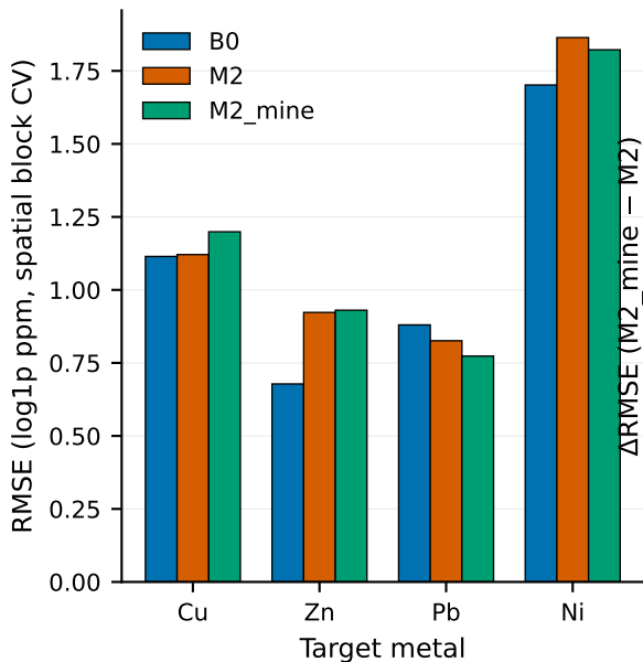
Spatial block CV RMSE
