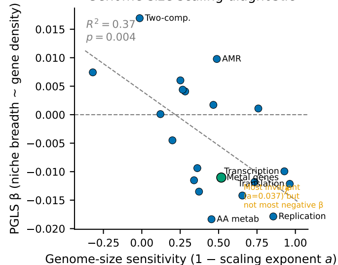
Genome-size scaling diagnostic
