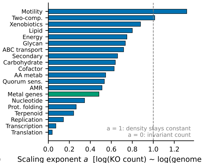
Gene count scaling with genome size
