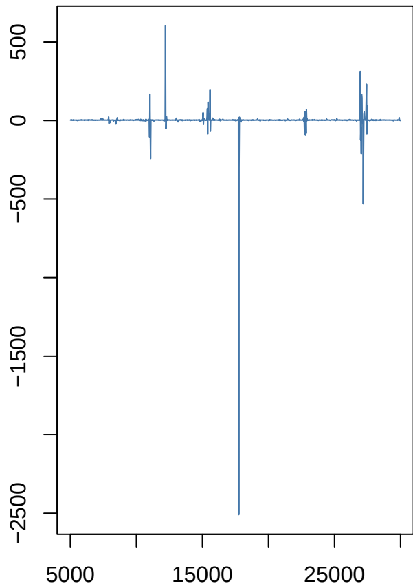
Trace: Intercept
