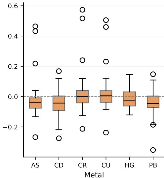
CSU pH control effect per metal
