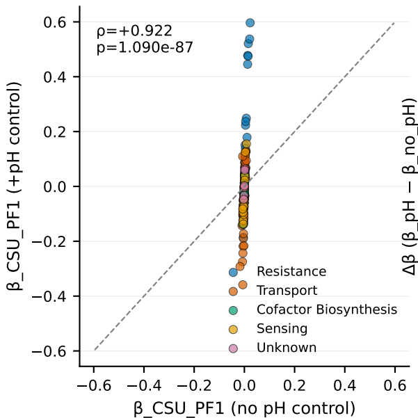
CSU \beta : no-pH vs pH-controlled
