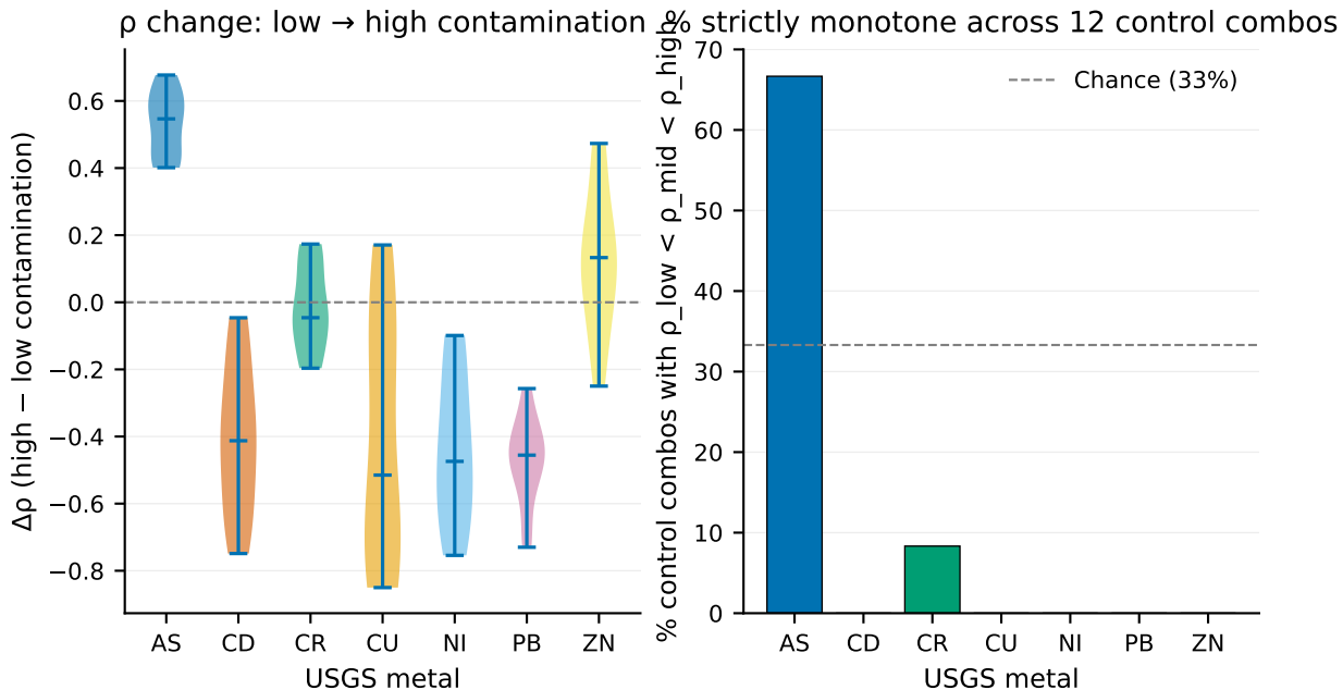
NB31 Fig 3: Does \lambda - \beta \rho increase with contamination level?
