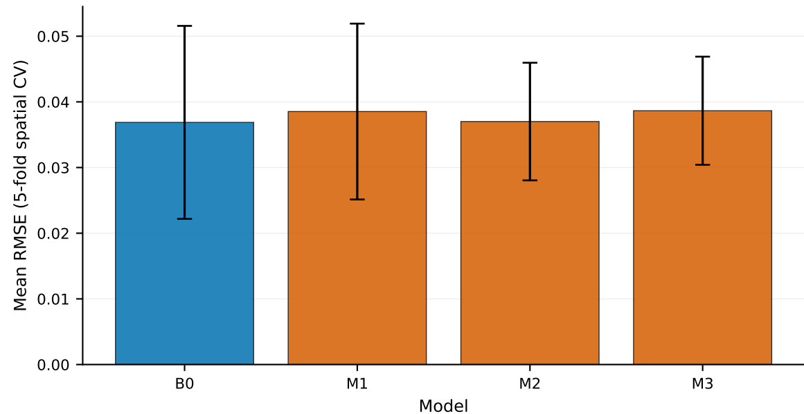
CV RMSE by model (MGnify) — target: PF1_Cu
