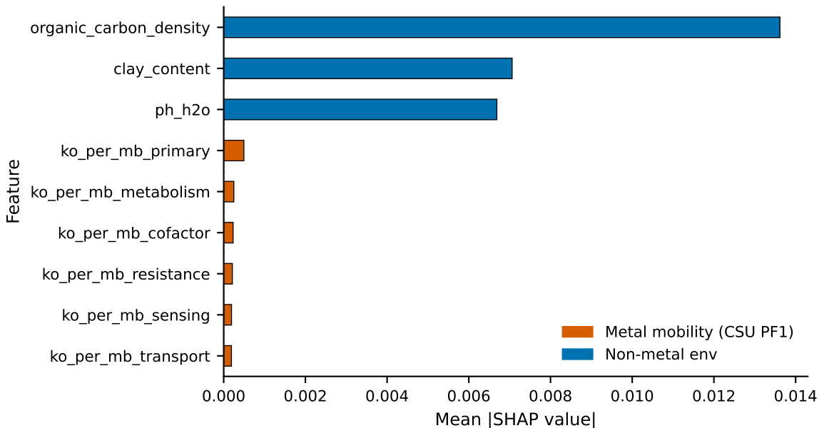
M3 SHAP importance (MGnify) — target: PF1_Cu
