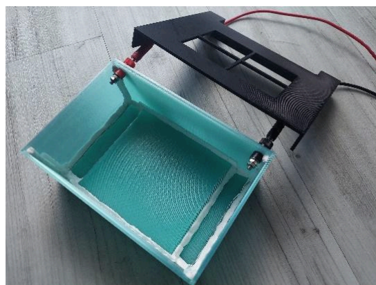
Completed EZ-Phoresis assembly.
