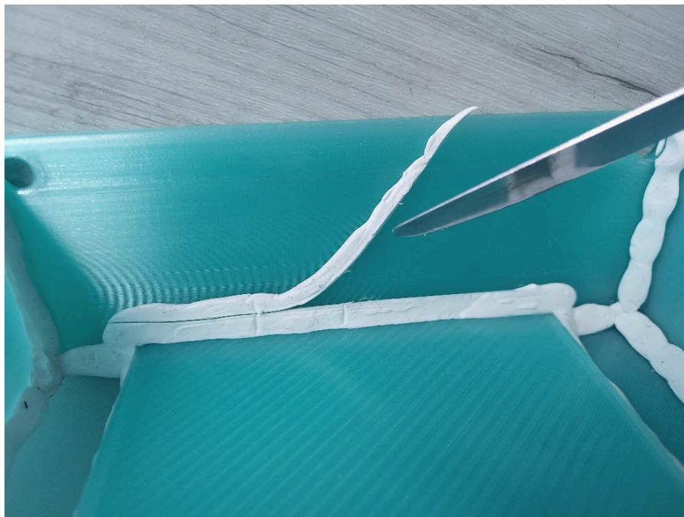
Example of a smoothed silicone seam.
